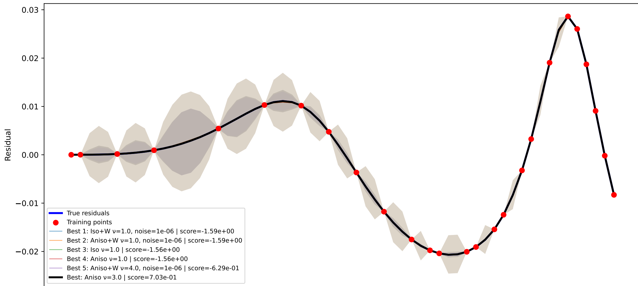
GPR kernel comparison node=7 RMSE=4.284e-06, train RMSE=2.813e-11
